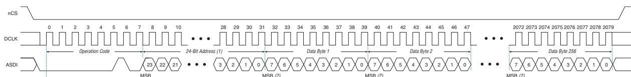
Figure 4-14. Write Bytes Operation Timing Diagram
